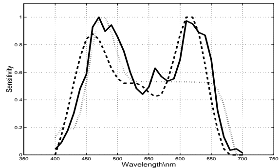
Figure 4: Recovered blue sensor for the Kodak DCS460 digital camera. The measured sensor (solid line) is shown together with an estimate constrained to be uni-modal (dotted line) and an estimate without this constraint (dashed line). Each sensor is normalised such that its maximum sensitivity is 1.
