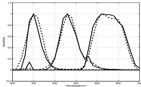
Figure 5: Recovered sensors for a colour scanner. The actual sensors (solid lines) are shown together with the recovered sensors (dashed lines). Each sensor is normalised such that its maximum sensitivity is 1.
