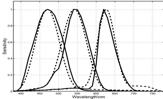
Figure 2: Recovered sensors for a digital camera. The measured sensors (solid lines) are shown together with the recovered sensors (dashed lines). Each sensor is normalised such that its maximum sensitivity is 1.
