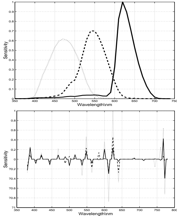
Figure 1: The sensor curves of a typical 3-band digital camera (top) and the sensors obtained by a simple linear regression (bottom).
