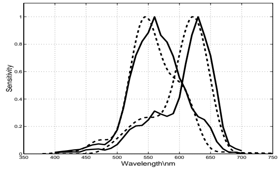
Figure 3: Recovered red and green sensors for the Kodak DCS460 digital camera. The measured sensors (solid lines) are shown together with the recovered sensors (dashed lines). Each sensor is normalised such that its maximum sensitivity is 1.
